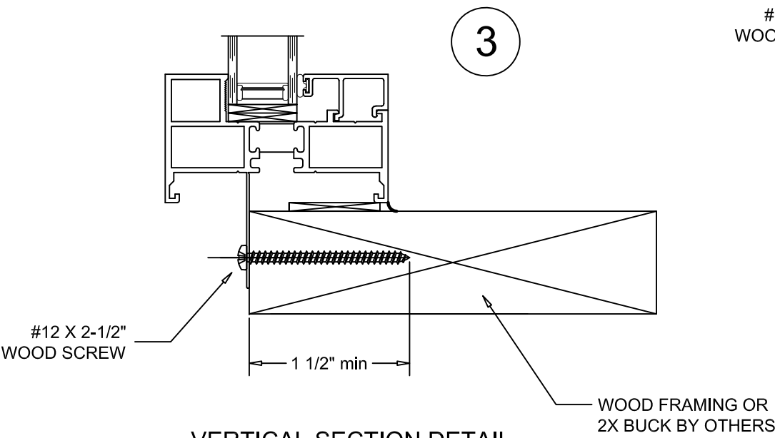
VERTICAL SECTION DETAIL WOOD FRAMING INSTALLATION
