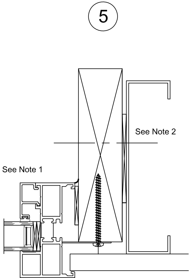
STEEL FRAMING INSTALLATION
