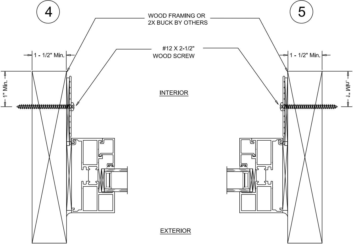
HORIZONTAL SECTION DETAIL WOOD FRAMING INSTALLATION
