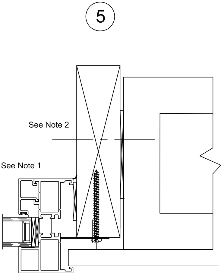
CMU INSTALLATION
