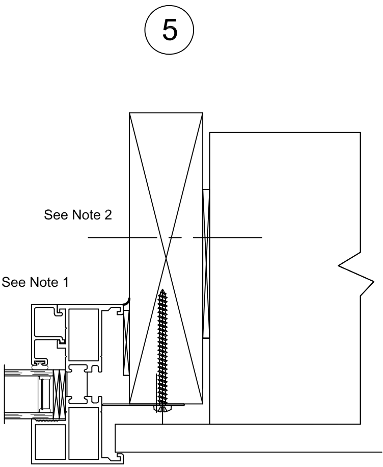
CONCRETE INSTALLATION
