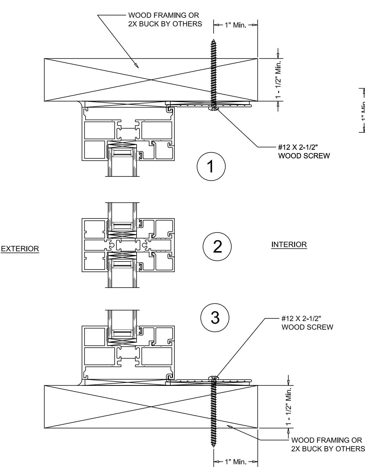
VERTICAL SECTION DETAIL WOOD FRAMING INSTALLATION
